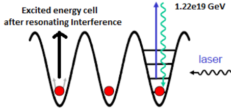
Figure 3: Illustration of probing the energy cell for information after the resonating interference. The red dot in the potential well illustrates an imaginary bit of information captured in the resultant energy cell after resonant interference.
